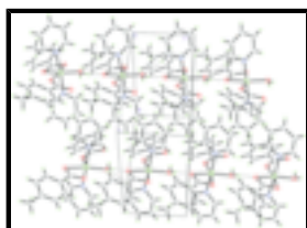
Fig. 2. The crystal packing of (I). The intermolecular hydrogen bonds are shown as dashed lines.
